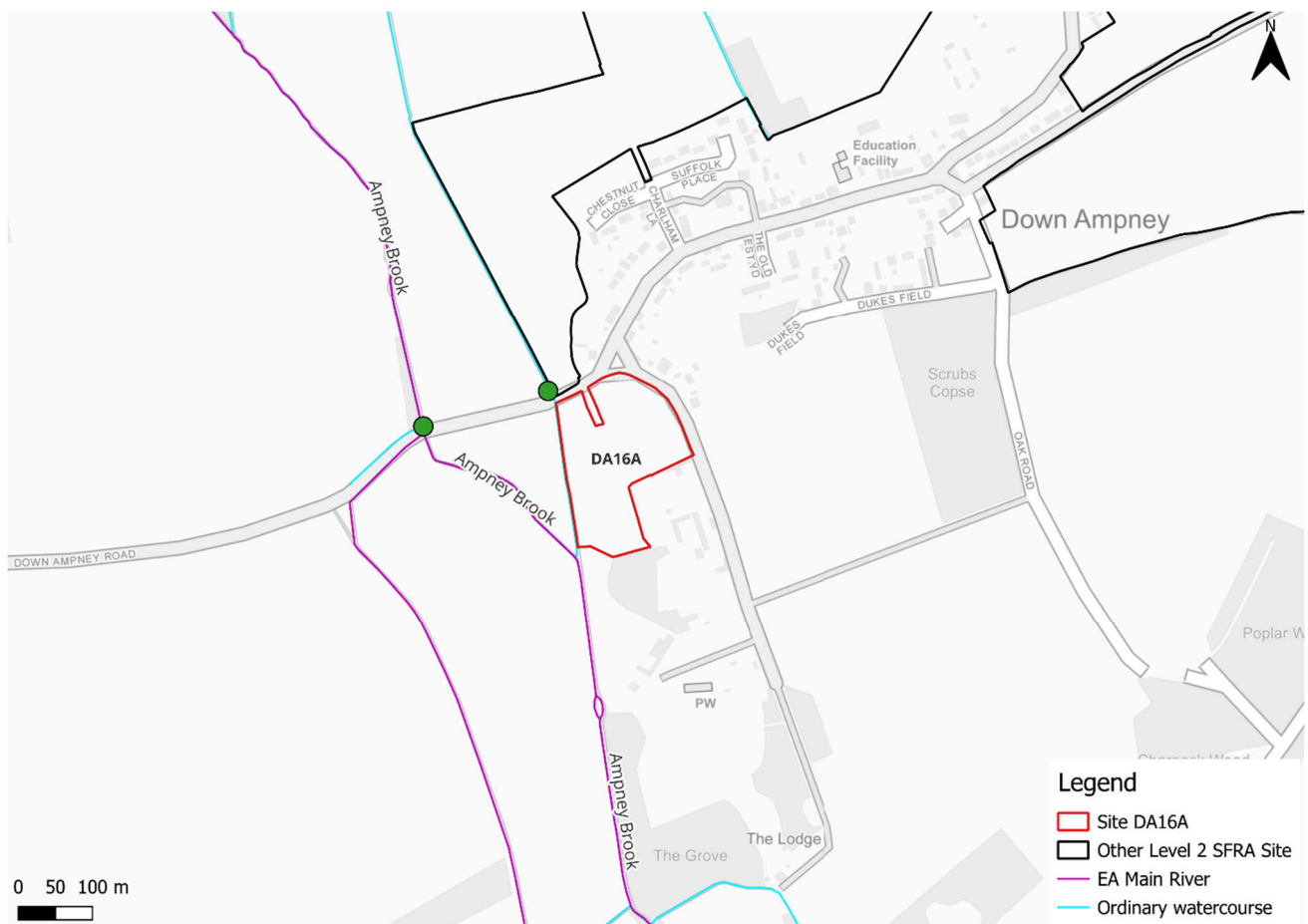
Figure 6-1: Culvert location (green circle)
