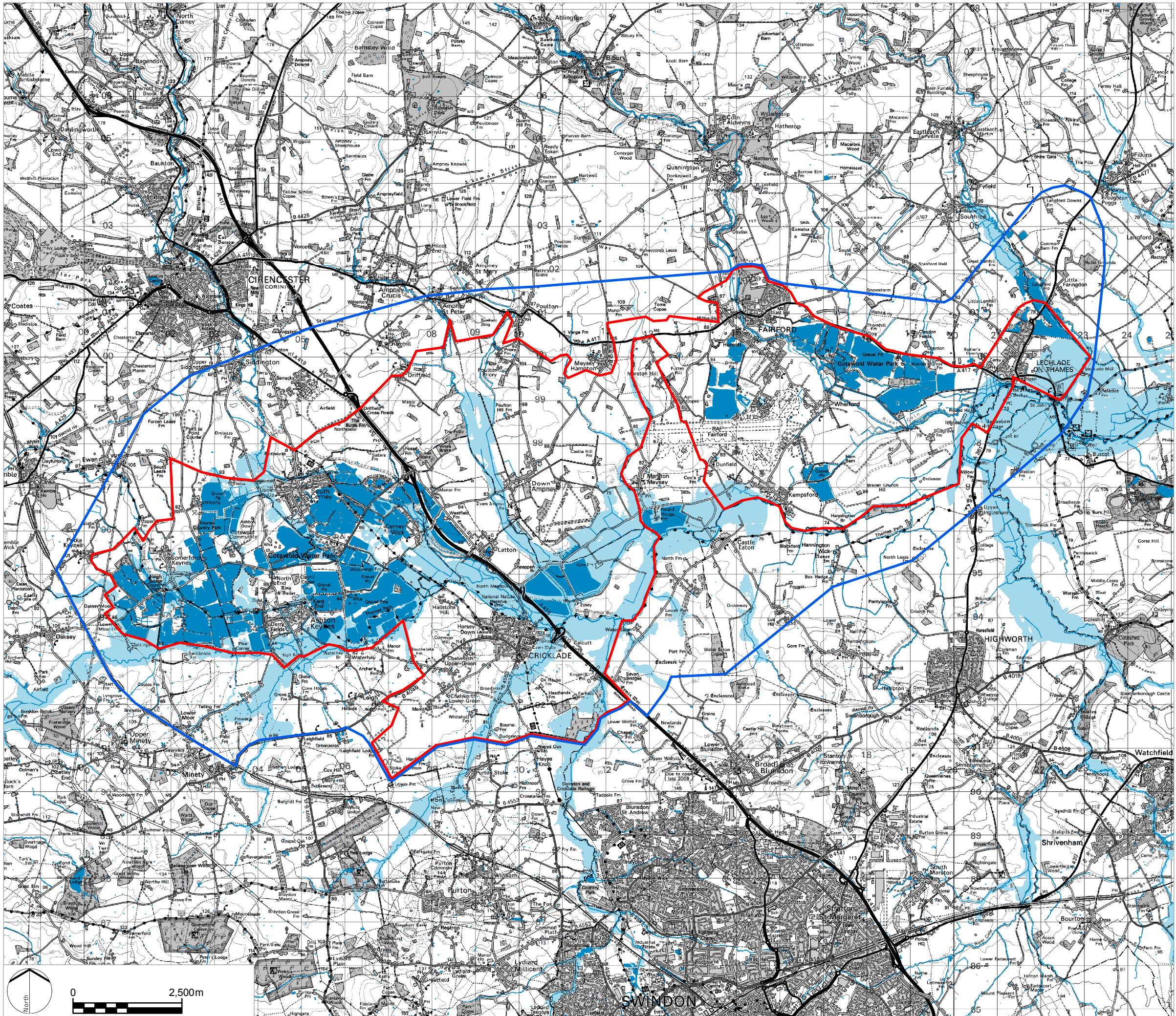
Figure 8: Hydrology
